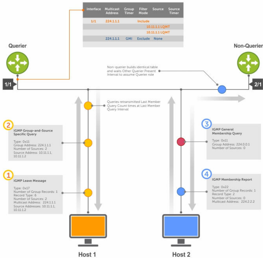
Figure 41. Membership Queries: Leaving and Staying
